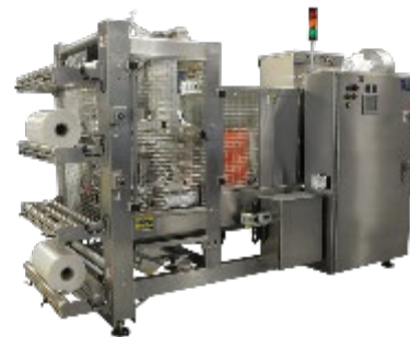
nVenia ARPAC Brand AGR Ice Cream Shrink Bundlers
